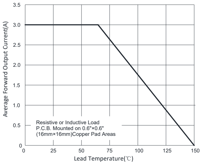
FIG1: Io-TL Curve
